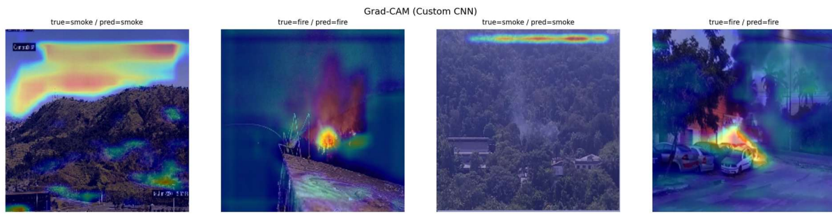
Figure 9 . Grad-CAM visualisation showing the model focuses on the flame region. Representative output.
