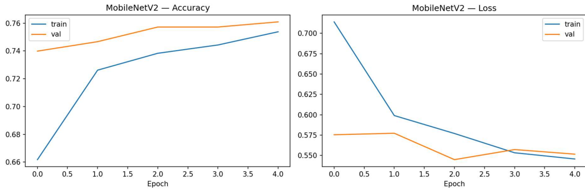
Figure 3. Training and validation accuracy/loss curves (MobileNetV2). Representative output.
