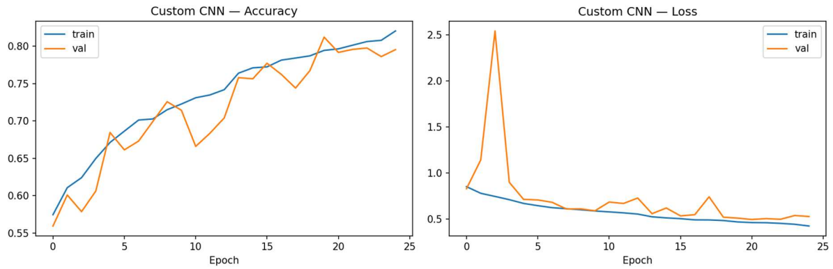
Figure 5. Training and validation accuracy/loss curves (CustomCNN). Representative output.
